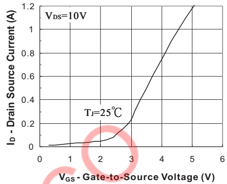
FIG.2- Transfer Characteristic
