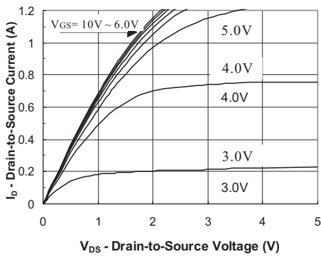
FIG.1- Output Characteristic
